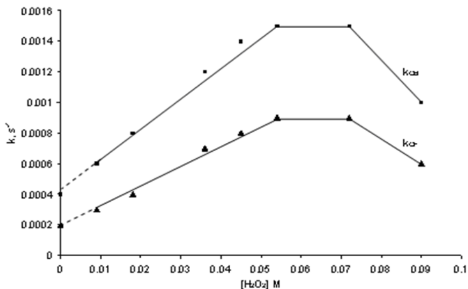
Fig.2. The influence of H 2 O 2 concentration on the rate constants k CB and k Cl - .
