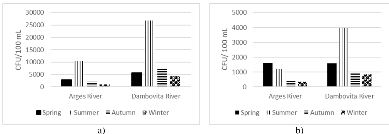
Fig. 2. Total coliforms (a) and E. coli (b) seasonal densities in Dambovitza and Arges rivers
