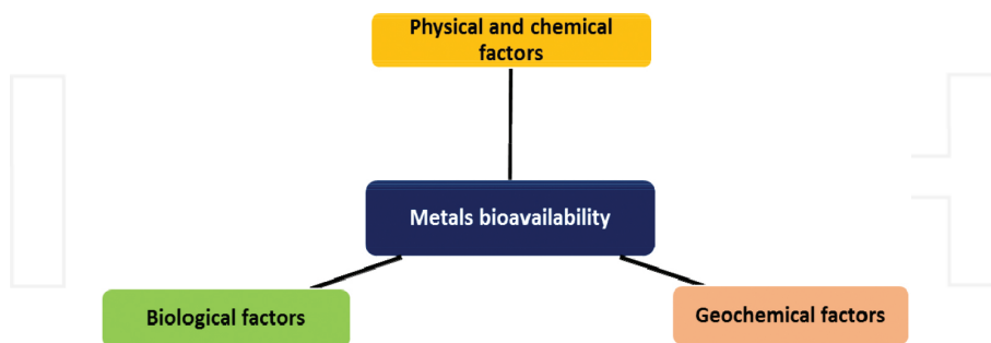
Figure 2. The main control factors that influence metal bioavailability.
