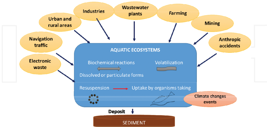
Figure 1. Sources of metal contamination affecting aquatic ecosystems.
