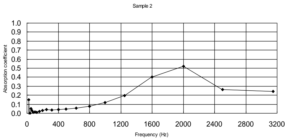
Fig. 2 - Coeficientul de absorbtie pentru proba 2 (rășină poliesterică 20% + fulgi de PET 80%) / Absorption coefficient for sample 2 (20% polyester resin + 80% PET pellets).
