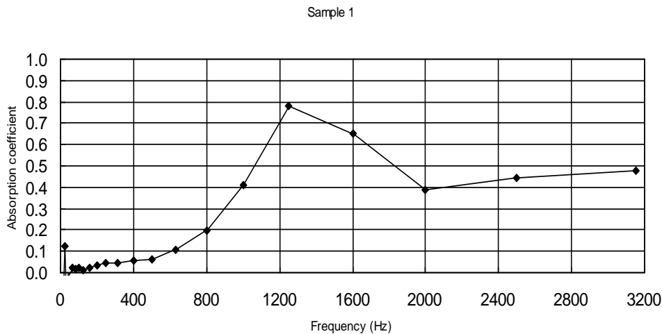
Fig. 1 - Coeficientul de absorbtie pentru proba 1 (rășină poliesterică 80% + talaj 20%) / Absorption coefficient for sample 1 (80% polyester resin + 20% wood chips).
