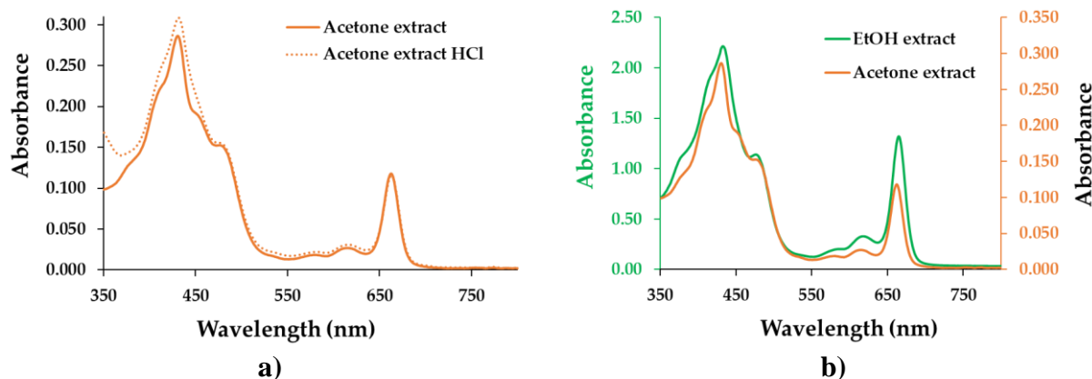
Figure 6. Recorded UV-Vis spectra for granular activated biomass extracts in a) acetone vs. acetone with 10 \mu\text{L} HCl 3M added to 10 mL extract and b) acetone extract vs. ethanolic extract
