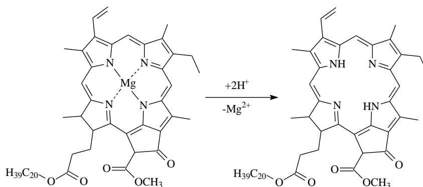
Figure 2. Chlorophyll to pheophytin transformation in acidic media.
