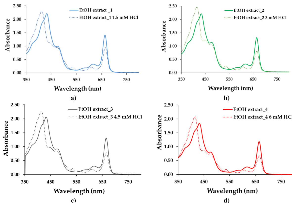
Figure 4. UV-Vis Spectra of ethanolic extracts obtained from microalgae biomass before (continuous lines) and after (dotted lines) acidification up to HCl concentrations of: a) 1.5 mM, b) 3.0 mM, c) 4.5 mM and d) 6.0 mM
