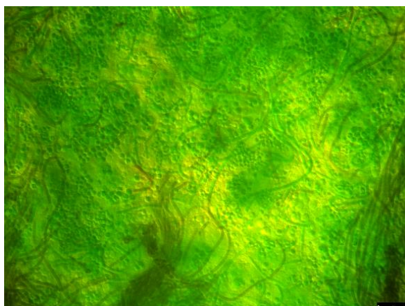
Figure 3. Light microscopy image of the microalgae populations distribution inside activated algae granules (200x magnification).
