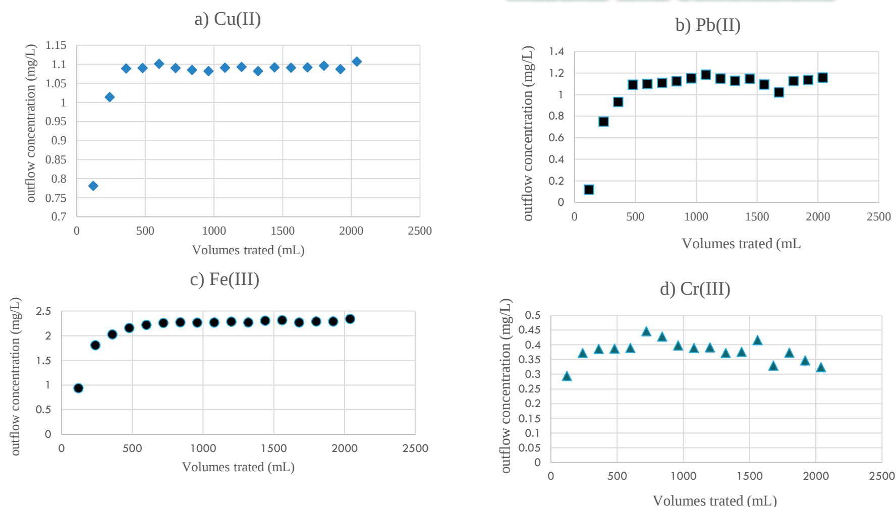
Figure 3. Concentrations of Cu(II), Pb(II), Fe(III), and Cr(III) in outflow
