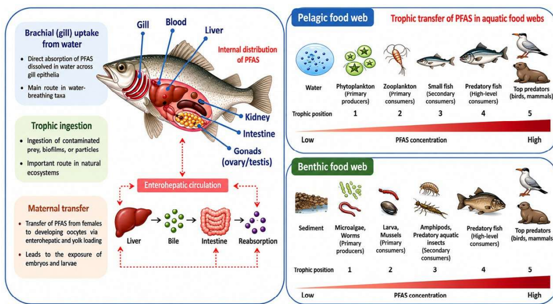
Figure 4. Integrated pathways of PFAS uptake, internal distribution, and trophic transfer in aquatic systems: coupling pelagic and benthic food web.
