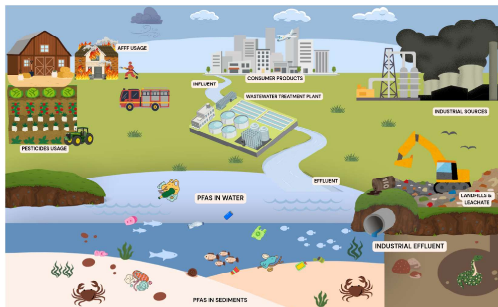
Figure 2. Sources, pathways, and environmental distribution of PFAS in aquatic systems.
