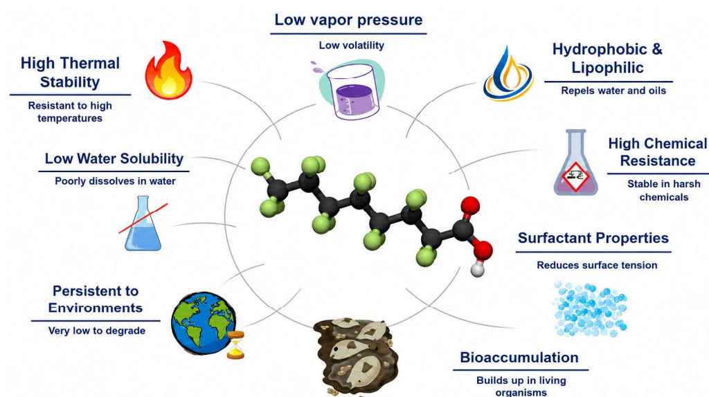
Figure 1. Physicochemical properties and environmental fate of PFAS.
