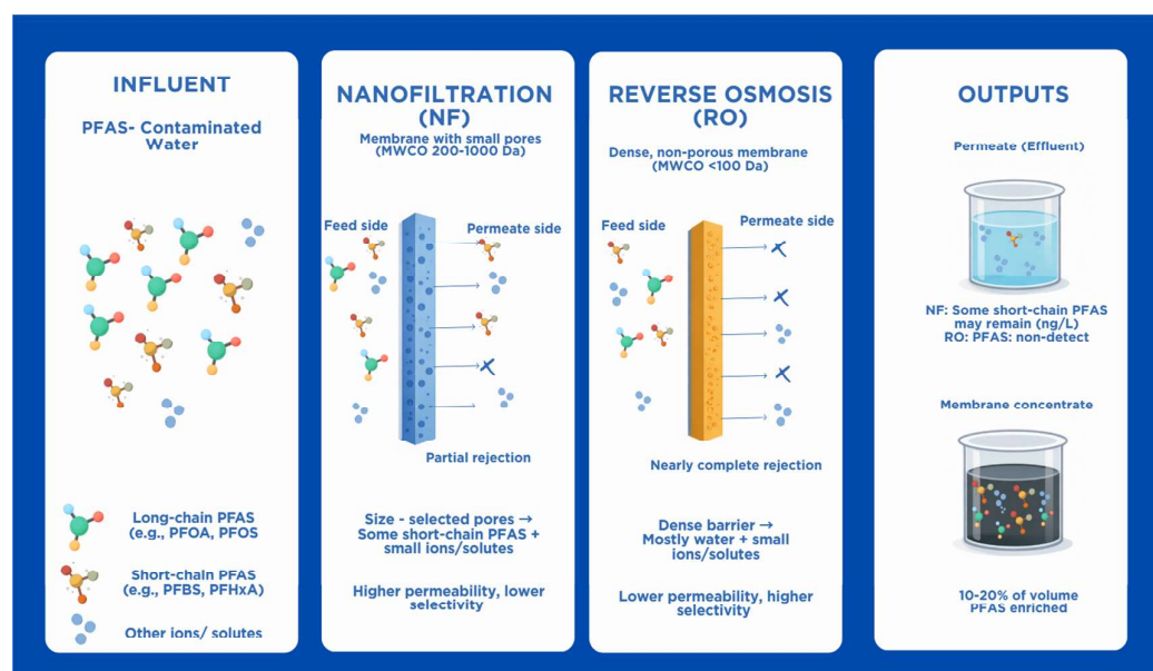
Figure 3. Nanofiltration and reverse osmosis processes for PFAS removal and their separation performance.
